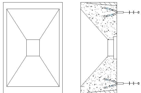
SECTION VIEW
